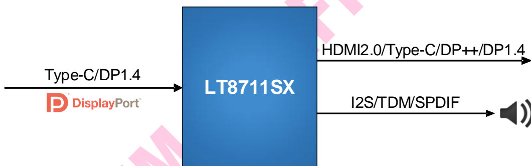
Figure 3.1. Application Diagram
