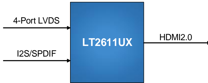
Figure 3.1 Application Diagram
