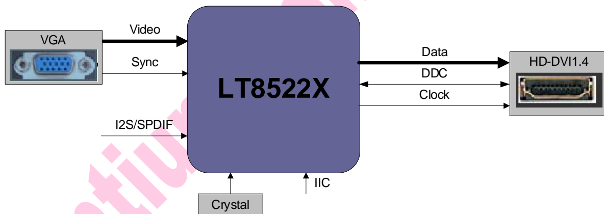
Figure 3.1 Application Diagram
