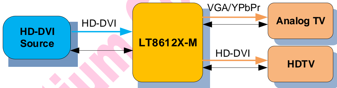
Figure 3.1 Application Diagram
