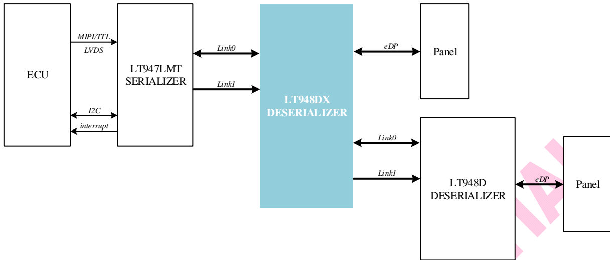
Figure 3.1 Application Diagram
