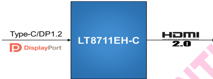
Figure 1. Application Diagram
