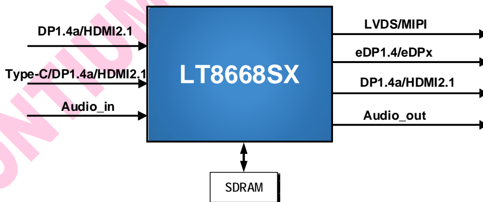
Figure 3.1 Application Diagram
