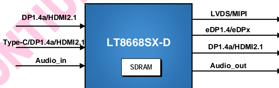
Figure 3.1 Application Diagram
