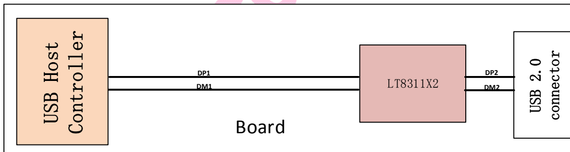
Figure 3.1 Application Diagram
