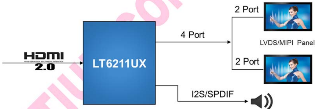
Figure 3.1 Application Diagram
