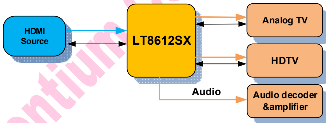
Figure 3.1 Application Diagram
