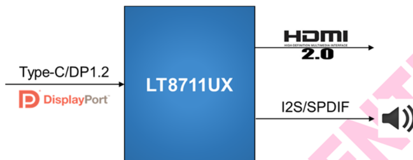
Figure 3.1 Application Diagram
