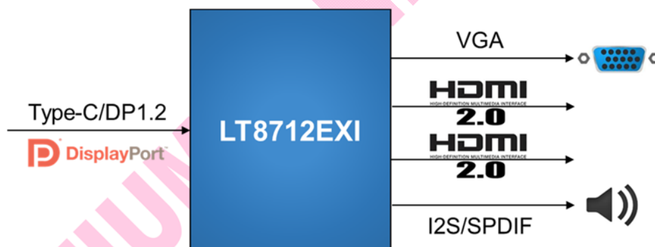
Figure 1. Application Diagram
