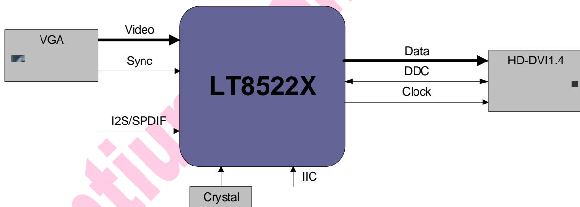
Figure 3.1 Application Diagram
