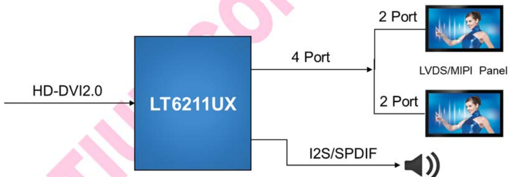
Figure 3.1 Application Diagram
